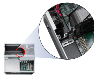
Customizable GPU Tail-End Retainer * Not included due to GPU dimension/screw holes are different from each other.
