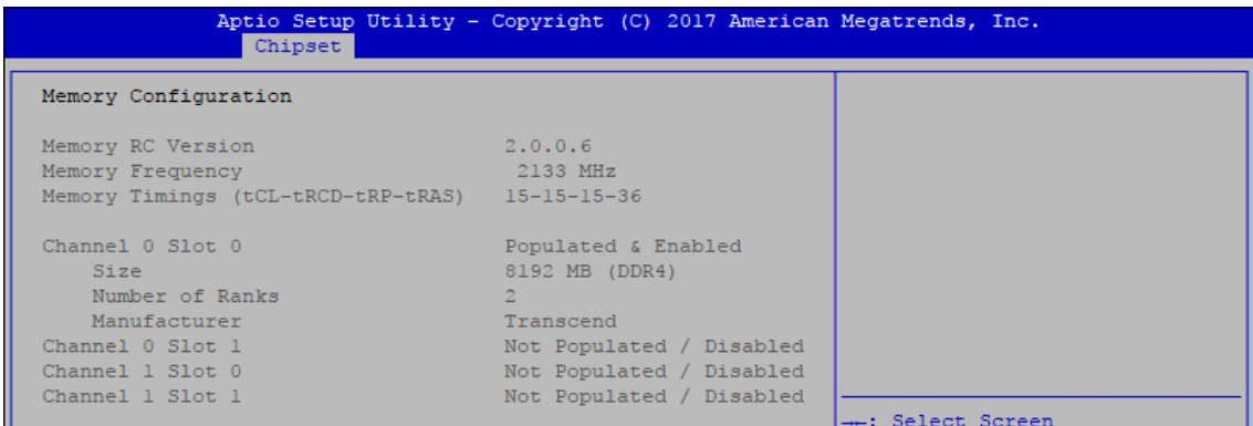
Figure 4-4-1-1 : Memory Information
