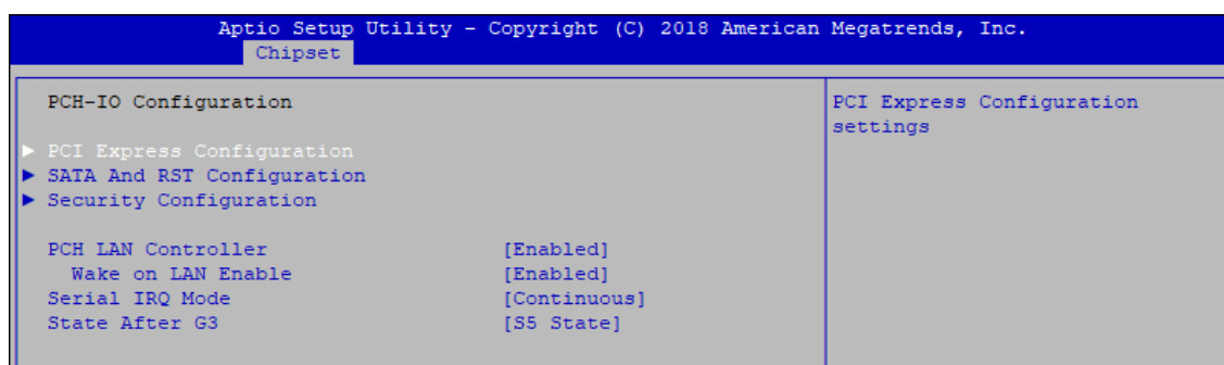
Figure 4-4-2 : PCH-IO Settings
