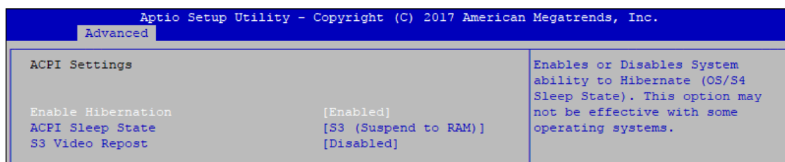
Figure 4-3-5 : ACPI Settings
