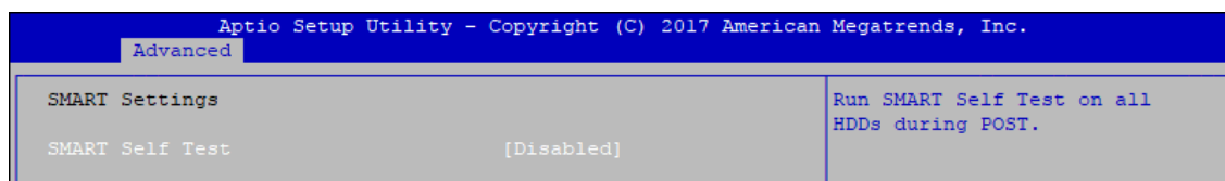
Figure 4-3-6 : SMART Settings
