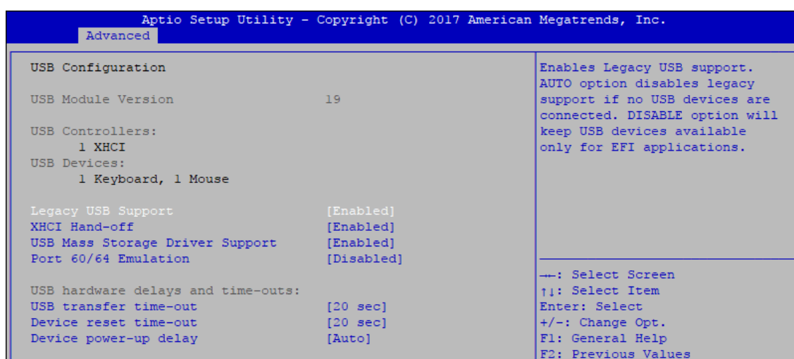
Figure 4-3-16 : USB Settings
