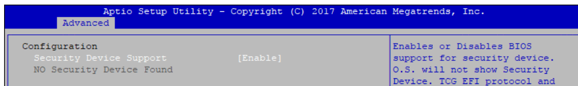
Figure 4-3-4 : Trusted Computing
