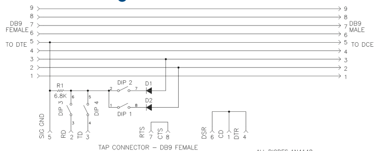
TAP CONNECTOR – DB9 FEMALE
