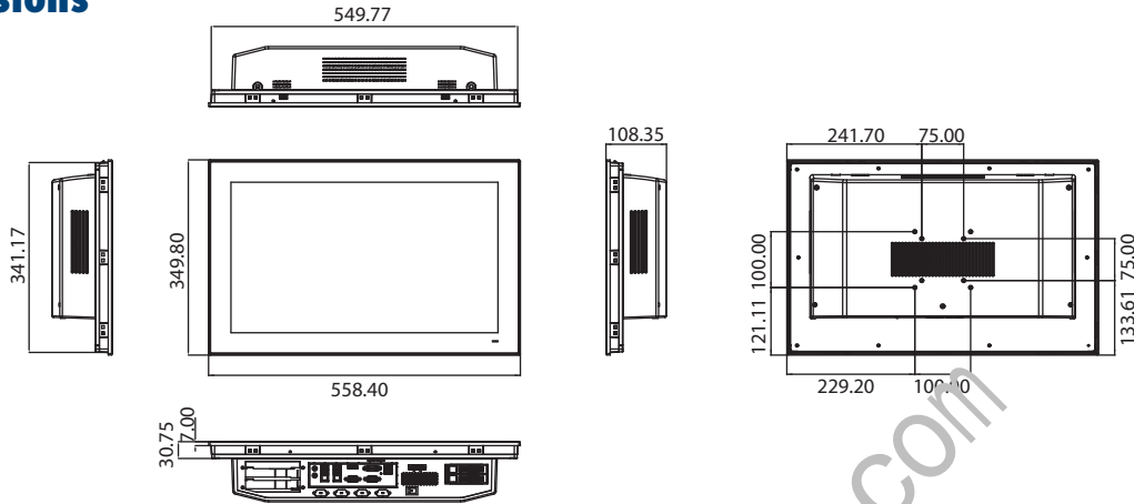
Panel Cutout Dimensions: 550.3 x 341.8 mm (21.65 x 13.45 in)
